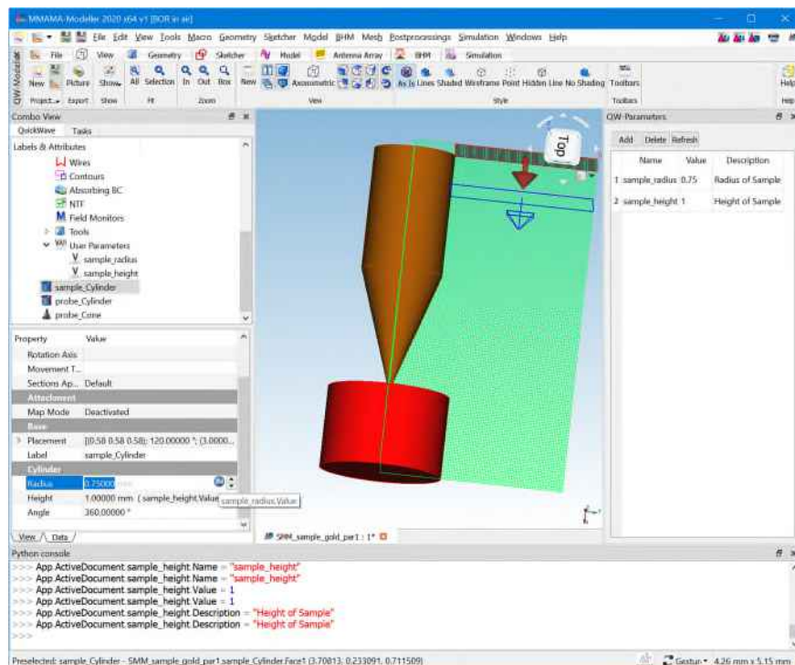
Fig. 4: A parameterised tip-sample example in MMAMA-Modeller: before tip radius change.
