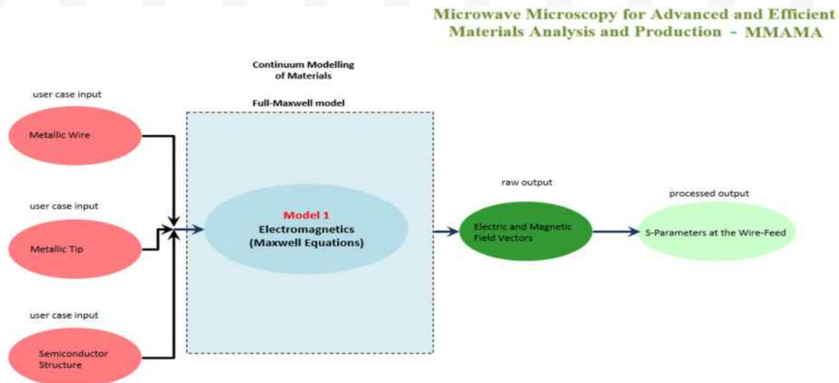
Fig.18: User Case 1: SMM tip (as discussed above; presented in [8][10]).
